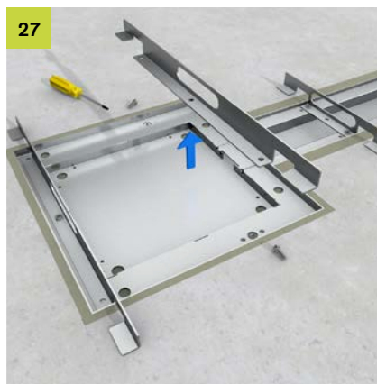
Remove levelling beams after the grout has cured. For information on the walkability of the grout, please refer to the manufacturer's information.
