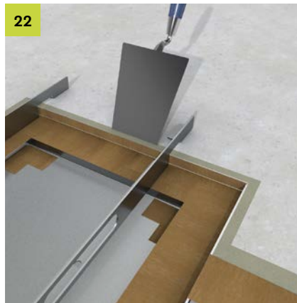
In order to avoid air inclusions and to distribute the grout optimally, „re-punching“ along the channel and cassette wings is recommended.
