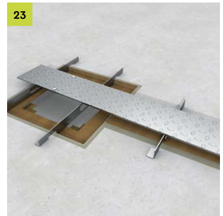
Weight down the cassette and channel, e.g. with a cover, to prevent flooding.
