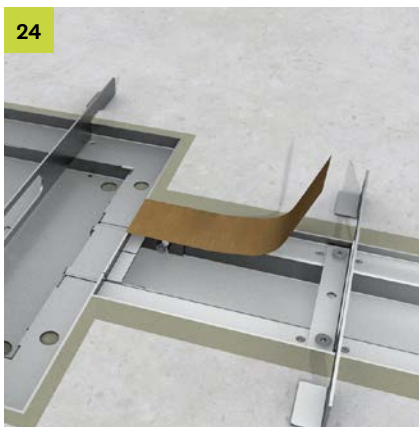
When the grout has reached its flow strength, remove the adhesive strip and clean the system and the surrounding floor.
